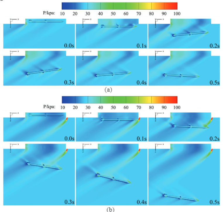
Figure 2. Pressure distribution contours in the symmetry plane: (a) Without wedge control and (b) With wedge control ( \Delta x = 0.09375w , \Delta z = 0.1875w , W = 1w ).
