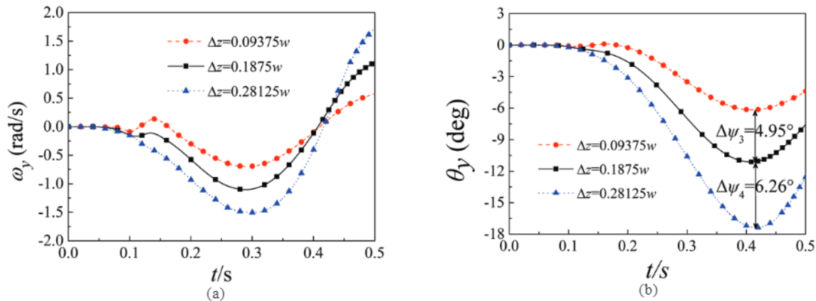
Figure 9. Variation of pitch angular velocity and pitch angle of the missile: (a) Pitch angular velocity and (b) Pitch angle.
