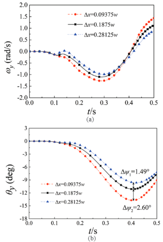
Figure 6. Variation of pitch angular velocity and pitch angle of missile: (a) Pitch angular velocity and (b) Pitch angle.
