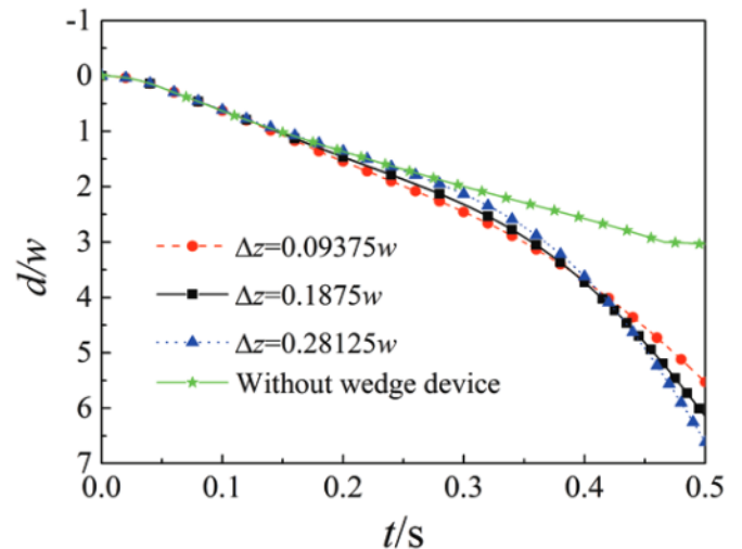
Figure 10. The minimum distance between the missile and the aircraft.
