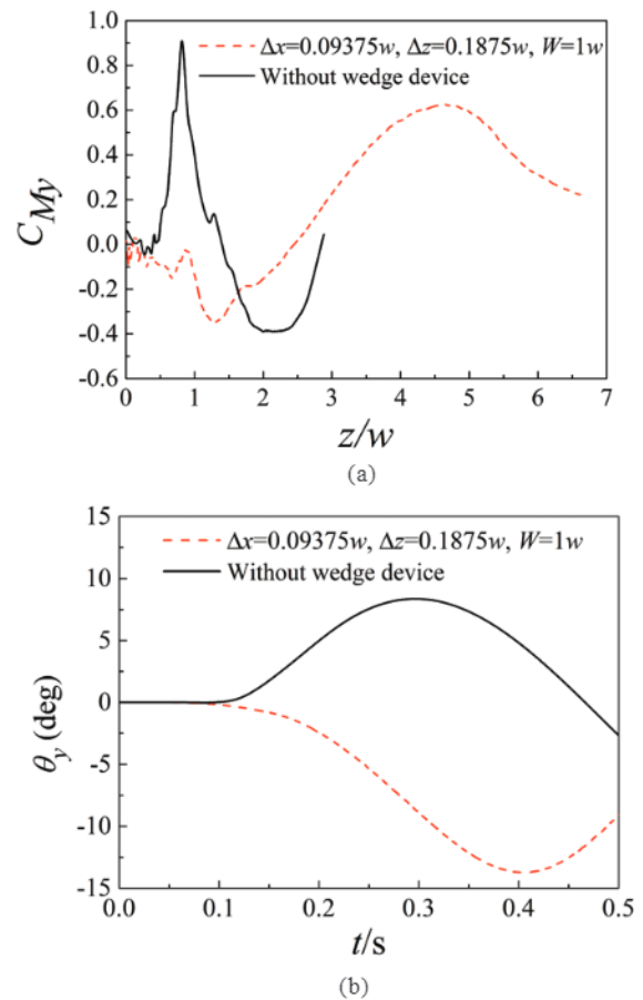
Figure 4. Pitching moment coefficient and pitch angle of missile: (a) Pitching moment coefficient and (b) Pitch angle.
