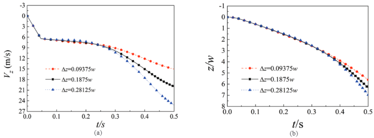
Figure 8. CG velocity and CG location of missile in the z direction: (a) CG velocity and (b) CG location
