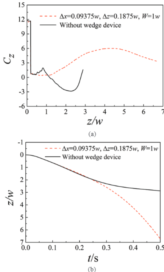
Figure 3. Force coefficient and CG location of missile in the z direction: (a) Force coefficient and (b) CG location.
