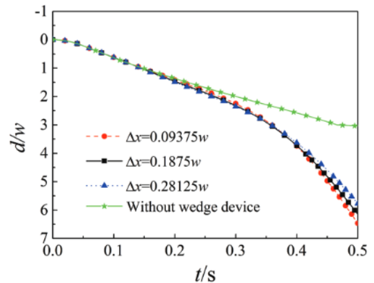
Figure 7. The minimum distance between the missile and the aircraft.
