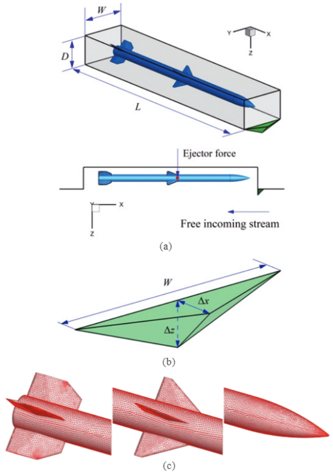
Figure 1. Geometric model and mesh (a) Geometric model, (b) Wedge device, and (c) Mesh distribution of missile.
