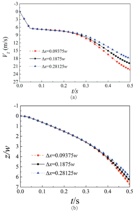
Figure 5. CG velocity and CG trajectory of missile in the z direction: (a) CG velocity and (b) CG trajectory.
